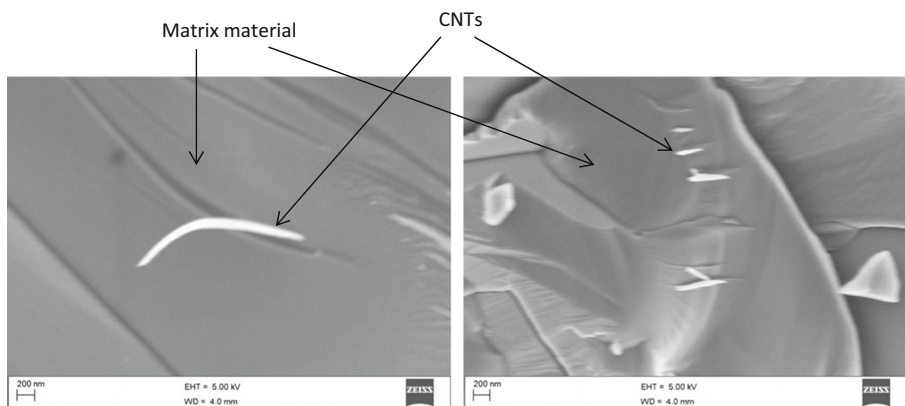
Fig. 2 SEM images of fractured cross sections of composite samples produced by laser sintering of chromium carbide powders and CNTs (0.5 wt.%)
