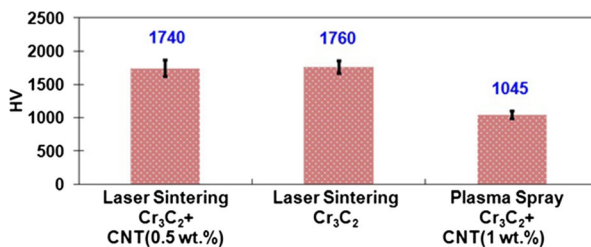
Fig. 5 (1) Hardness of composites produced by laser sintering of chromium carbide powders+CNTs (0.5 wt.%), (2) hardness of material produced by laser sintering of chromium carbide powders without CNTs, and (3) hardness of composites produced by plasma spraying of chromium carbide powders+CNTs (1 wt.%) taken from [4]
