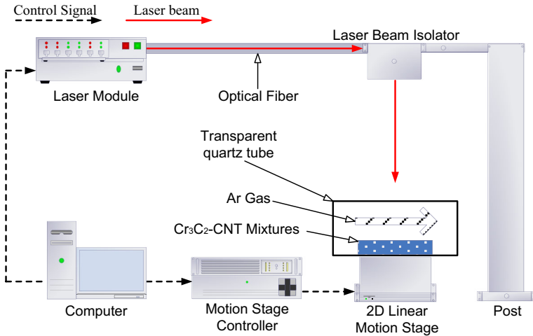
Fig. 1 Schematic diagram of the experimental setup (some components are not shown)
