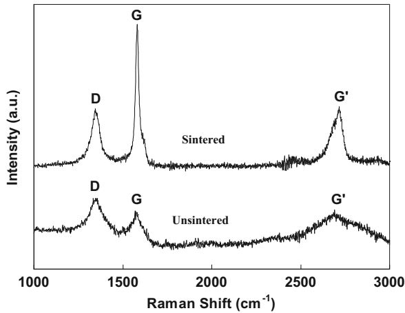
Fig. 3 Raman spectrum for an un-sintered mixture sample of CNTs (0.5 wt.%) and chromium carbide powders ( lower ), and for a laser-sintered composite sample ( upper ) (each spectrum clearly shows the G, D, and G' peaks [9–12])
