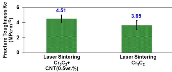
Fig. 6 Vickers indentation fracture toughness of (1) composites produced by laser sintering of chromium carbide powders+CNTs (0.5 wt.%), and (2) material produced by laser sintering of chromium carbide powders without CNTs
