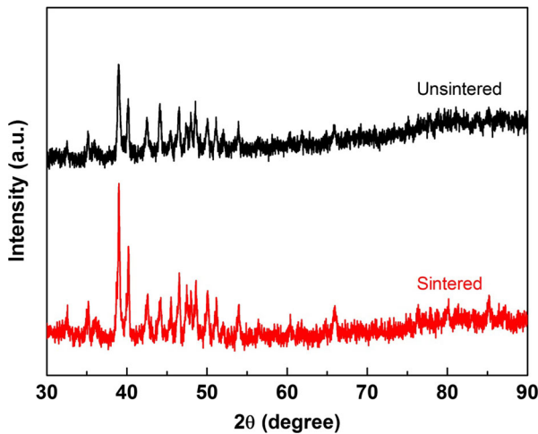
Fig. 4 XRD spectrum for an un-sintered mixture sample of CNTs (0.5 wt.%) and chromium carbide powders ( upper ), and for a laser-sintered composite sample ( lower )
